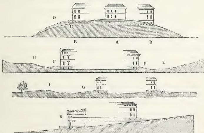
[Fig. 24. Sections to shew the manner of adapting houses to different natural shapes of ground.]
